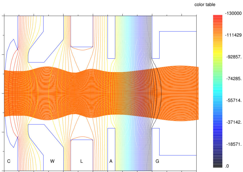
Figure 2: Electron gun with cathode (C), a Wehnelt electrode (W) to control the current, an einzel lens (L) to match the beam to the acceleration gap between anode (A) and ground (G). Potential lines are displayed together with electron trajectories.
