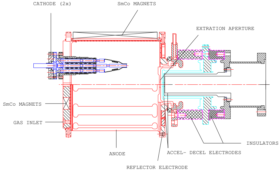
Figure 7: MUCIS multi cusp ion source
