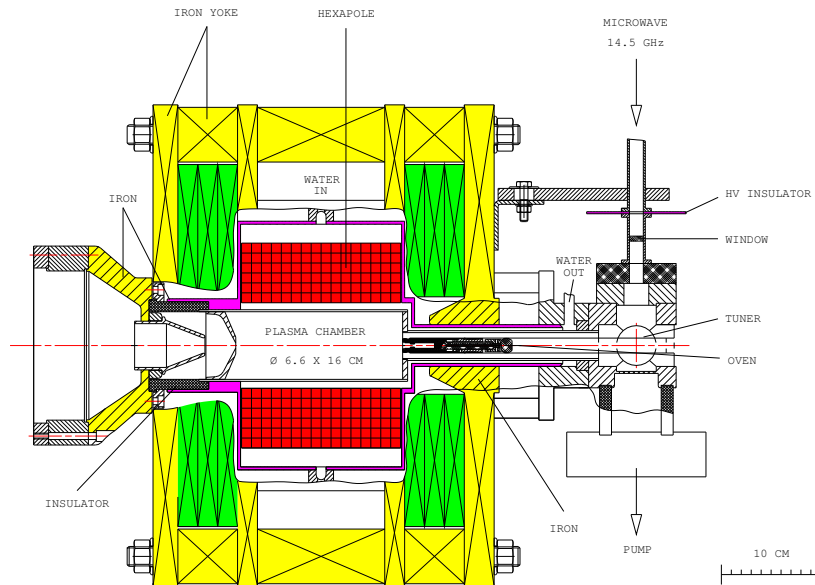
Figure 8: CAPRICE ion source.
