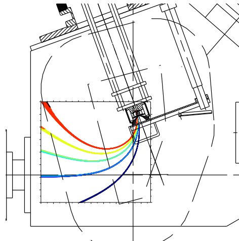
Figure 13: Top view of a PIG source with an extraction system inside a 110^0 source dipole magnet, and the vacuum beam line. The rectangular insertion shows the region of computation together with an extracted Argon beam with charge states 1 to 5. Charge state 2 has been selected for the accelerator. A fully space charge compensated beam is assumed.
