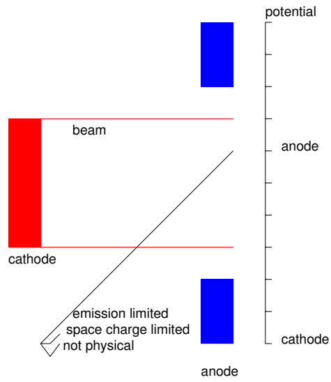
Figure 1: Potential on mid axis in front of the cathode for the three different current densities.
