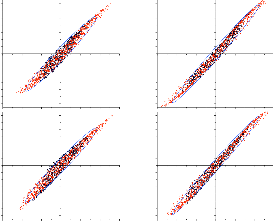
Figure 23: Influence of compensation behind the screening electrode on the beam divergence. Scaling is \pm 150 mrad and \pm 30 mm; left: compensated beam, right: uncompensated beam (3 mA at 12.5 keV). Top: vertical, bottom: horizontal.
