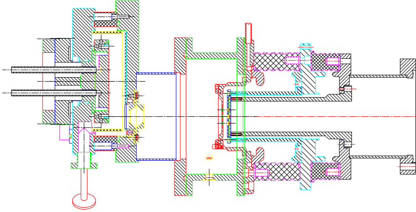
Figure 15: Mevva ion source
