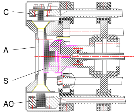
Figure 12: Side view of a Penning Ion Source with heated cathode (C), cold anti-cathode (AC), anode (A), and sputter electrode (S). The magnetic field points in the direction from cathode to anti-cathode.
