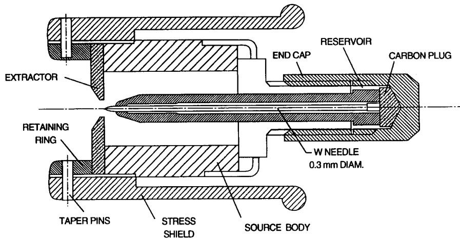
Figure 16: Laser Ion Source
