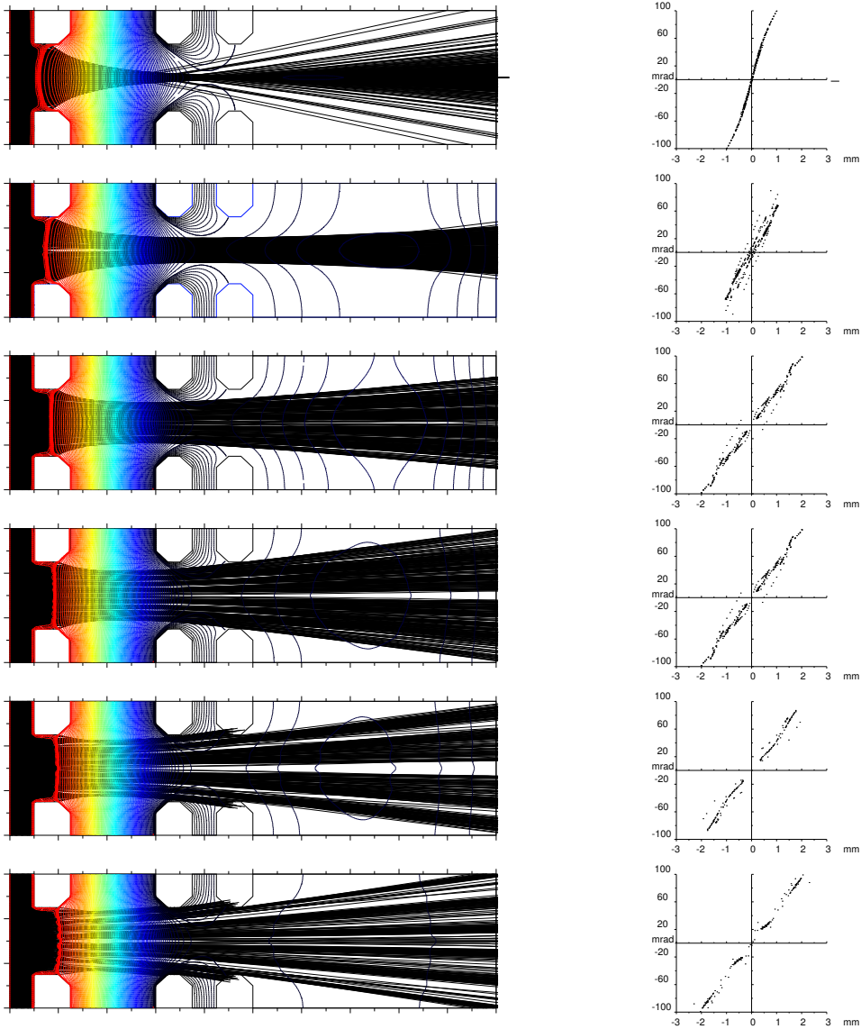
Figure 20: Computer simulation of the extraction with an accel-decel system. The current density within the plasma has been changed from 50 \text{ mA/cm}^2 (top) in steps of 50 \text{ mA/cm}^2 to 300 \text{ mA/cm}^2 (bottom). The plasma boundary is indicated by plotting a few potential lines between plasma potential and the potential of the plasma electrode.
