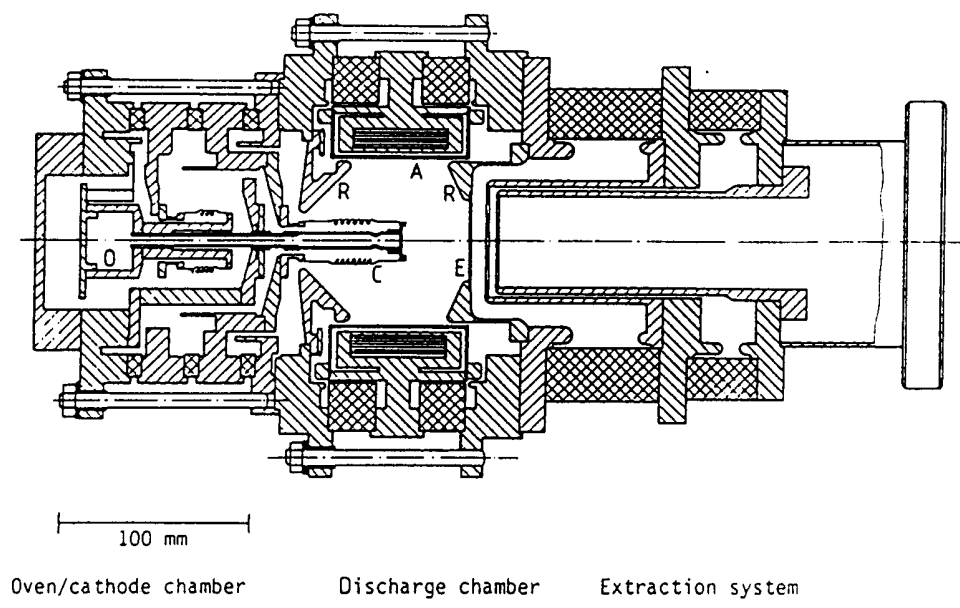
Figure 6: CHORDIS multi cusp ion source. Permanent magnets placed directly behind the anode (A) create a cusp field in radial direction. The cathode (C) is a hot filament cathode, reflector electrodes (R) confines the plasma electrostaticly. The oven (O) is used for non volatile elements. Extraction electrodes (E) are on the right.
