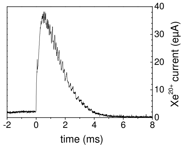
Figure 10: Analyzed current signal for the afterglow of \text{Xe}^{20+} . The rf power is switched off at time 0, releasing the trapped ions.
