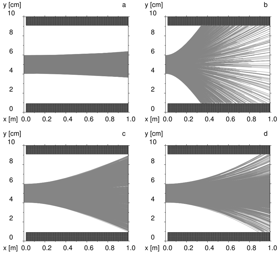
Figure 24: Beam envelope for a drifting beam: a) no space charge, b) full space charge, c) net current, and d) space charge compensation with the beam plasma model
