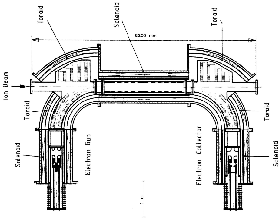
Figure 4: Electron cooler.
