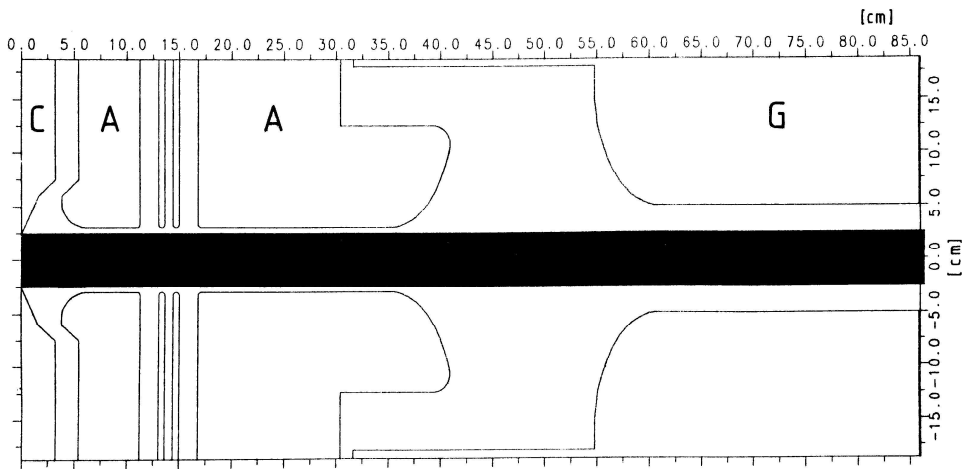
Figure 3: Electron gun with cathode (C), anode (A), and ground electrode (G). The anode is split in two different electrodes with two additional electrodes for optional resonant focusing.
