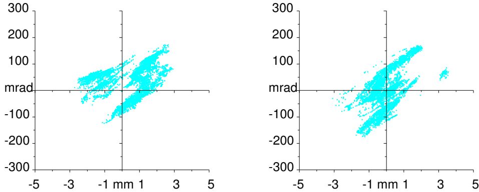
Figure 19: Both transverse emittances of the extracted ion beam, left \parallel \vec{B} , right \perp \vec{B} .
