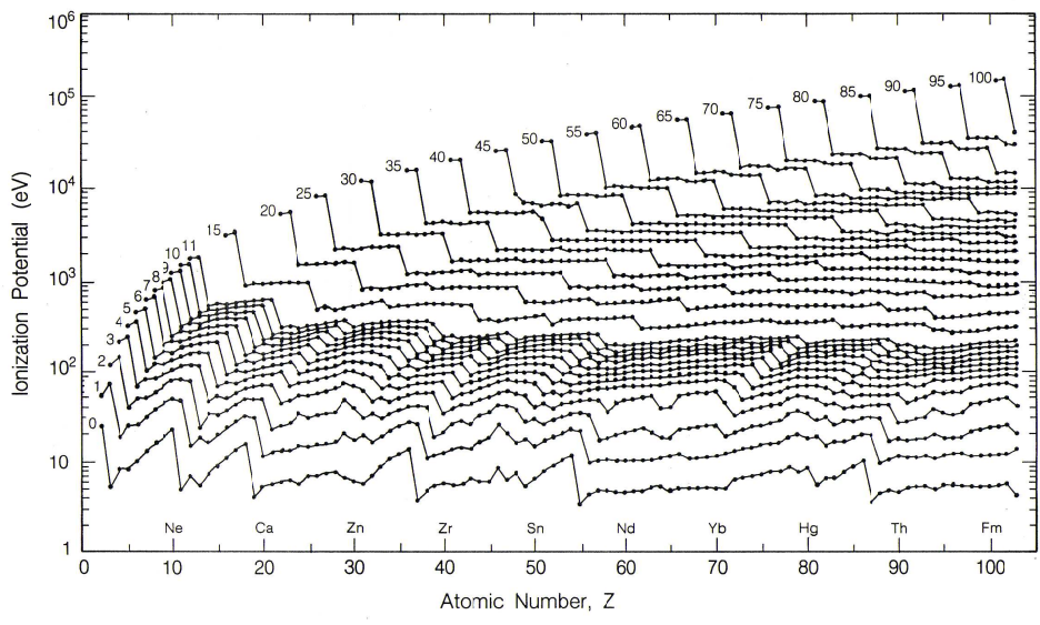
Figure 5: Ionization energies for different elements and different charge states.
