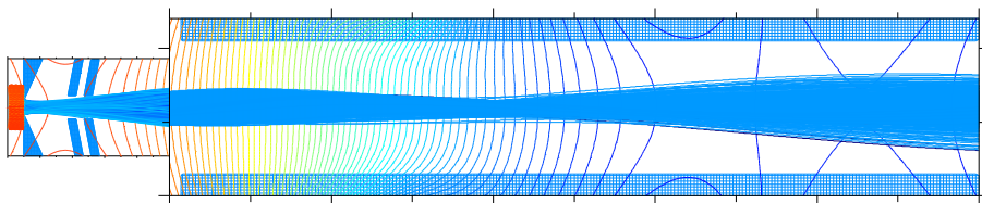
Figure 11: Geometry and lines of constant magnetic flux density in beam direction. The location of the maximum flux density is close to the negative screening electrode. Within the region of extraction the flux density drops from 3.3 T to 3.0 T, in the beam line a solenoidal lens focuses the beam
