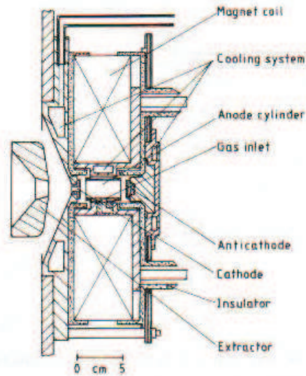
Figure 14: Penning Ion Source, axial extraction.
