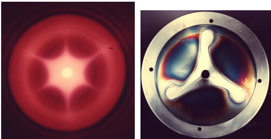
Figure 9: Radial shape of the plasma inside the plasma chamber (left) and sputter marks of the plasma on the plasma electrode (right).
