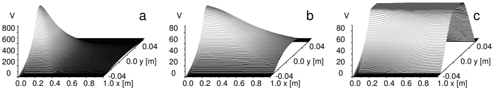
Figure 25: Space charge potential for a drifting beam: a) full space charge, b) net current, and c) space charge compensation with the beam plasma model
