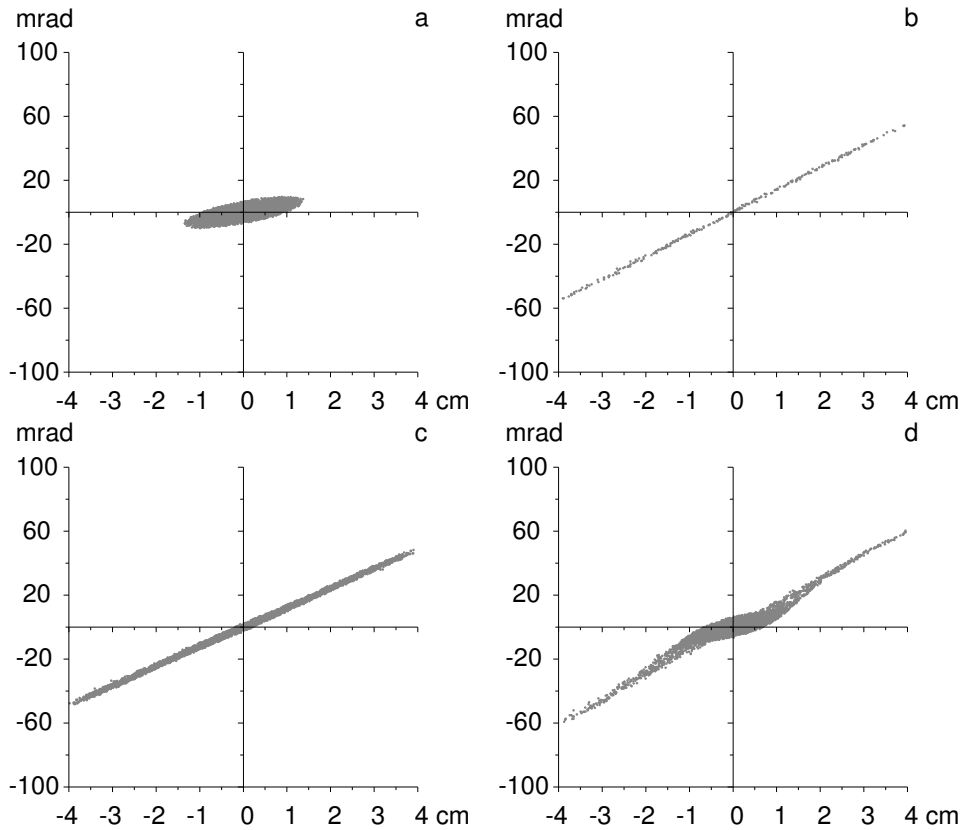
Figure 26: Beam emittance for a drifting beam: no space charge a), full space charge b), net current c), and space charge compensation with the beam plasma model d)
