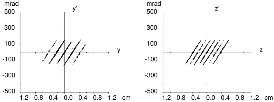
Figure 21: Emittance of a beam extracted by a multi aperture extraction system with 13 holes.
