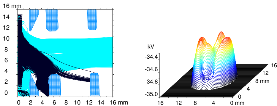
Figure 18: Beam envelope of the extracted ion beam under the influence of the magnetic filter field and tilted electrodes. Most electrons are trapped within the plasma, or dumped on the electrode. (left) However, if the plasma boundary is not perfectly matched, some electrons can be extracted. Potential perpendicular to the beam direction in front of the plasma electrode. The electrons bent out from the ion beam cause a nonlinear force. (right) Simulation made with KOBRA3-INP [11].
