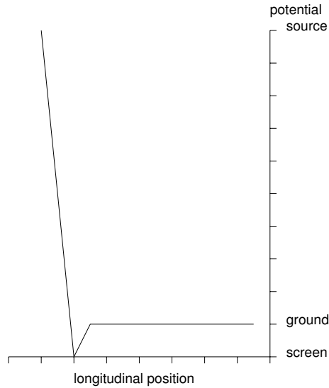
Figure 22: The negatively biased 2nd electrode has to produce a negative potential dip on axis of the extraction hole. This screens the electrons from acceleration towards the positive potential of the ion source.
