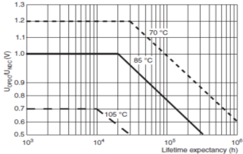
Lifetime expectancy – typical curve
