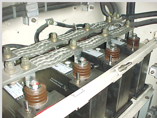
TGV input filter 1800VDC 8 mF
