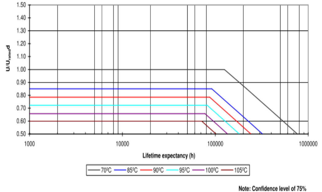
Life expectancy (typical curve)
