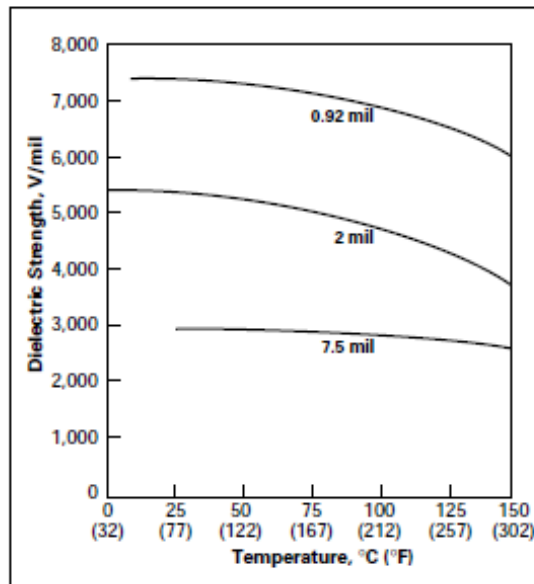
Figure 2. Dielectric Strength vs. Temperature
