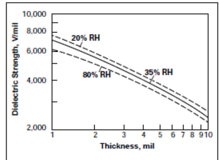
Figure 3. Dielectric Strength at Various Humidities
