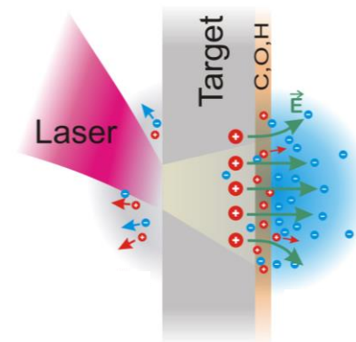
Laser-Plasma Ion acceleration
