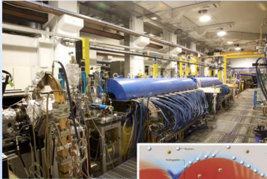
Plasma acceleration at SPARC_LAB experiment.
