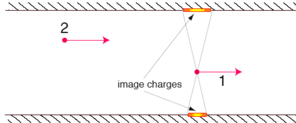
FIGURE 2. Particles traveling inside a perfectly conducting pipe of arbitrary cross section. Shown are the image charges on the wall generated by the leading charge.
