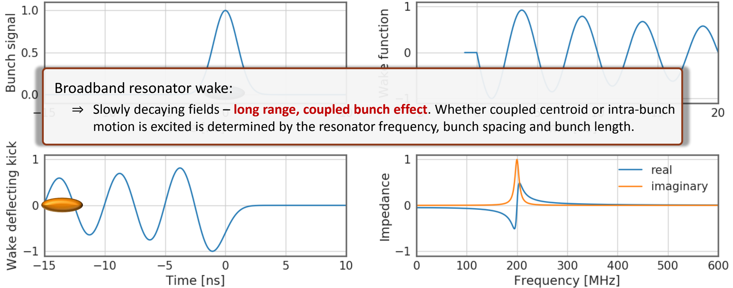
Gaussian bunch profile with \sigma = 1 ns
