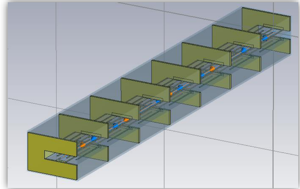
Serigraphed kicker
