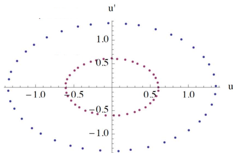
S 1 \alpha=0
