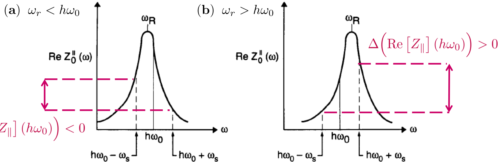
Figure 4.4. Illustration of the Robinson stability criterion. The rf fundamental mode is detuned so that \omega_R is (a) slightly below h\omega_0 and (b) slightly above h\omega_0 . (a) is Robinson damped above transition and antidamped below transition. (b) is antidamped above transition and damped below transition.
