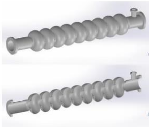
An SRF technology 9-cell Nb cavity
